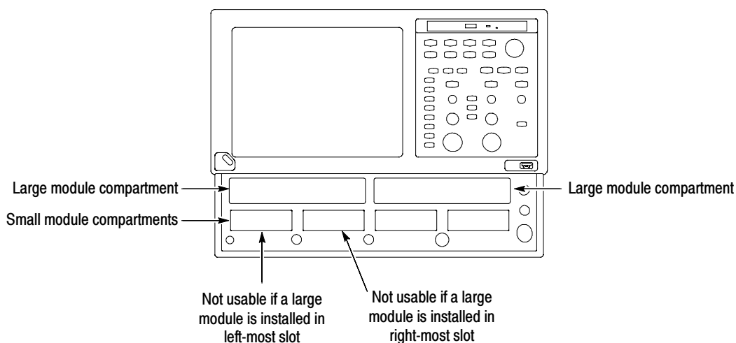
Figure 3: Module compartments
